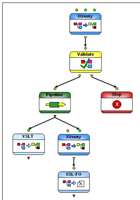
Figure 419. Diagram of getHoldings.pipeline
