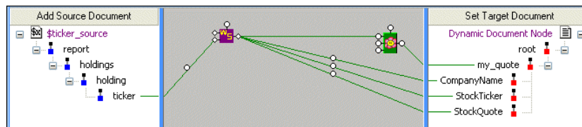
Figure 390. Finished Mapping
