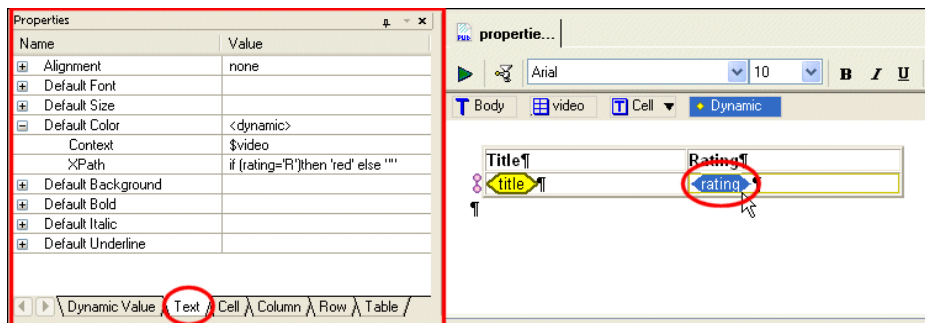
Figure 510. Properties Window
