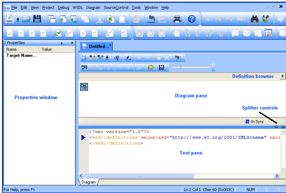
Figure 407. WSDL Editor
