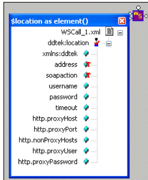
Figure 380. ddtek:wscall Location Input Port
