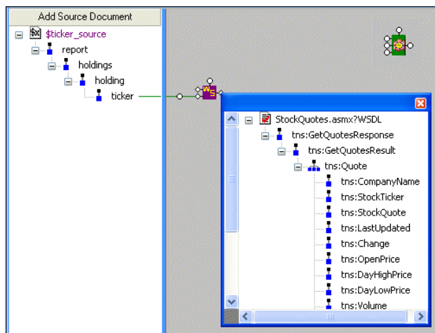
Figure 388. Selecting Output
