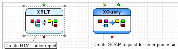
Figure 458. Pipeline Labels
