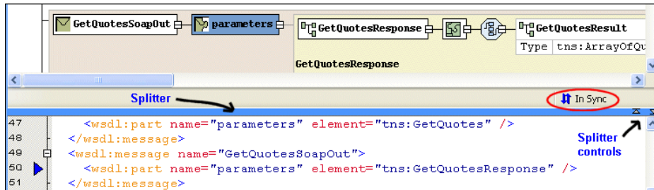
Figure 409. Diagram and Text Panes in the WSDL Editor
