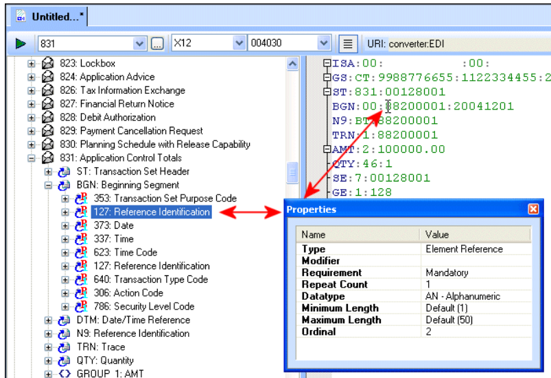
Figure 220. Properties Window
