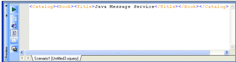
Figure 350. Predicate Result
