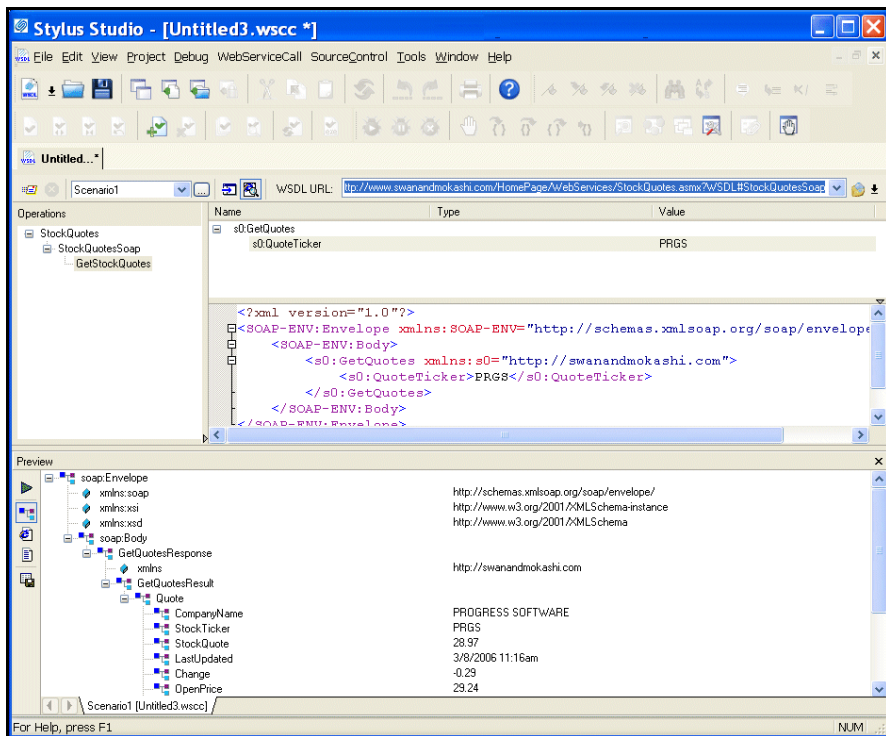
Figure 397. SOAP Response
