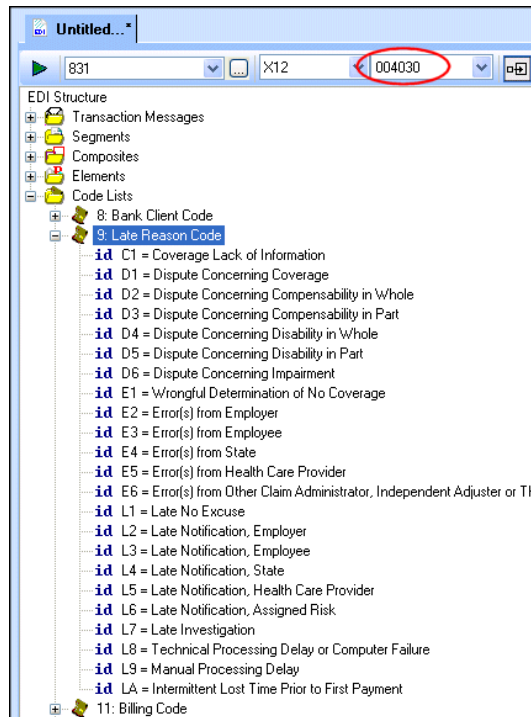
Figure 221. EDI Structure
