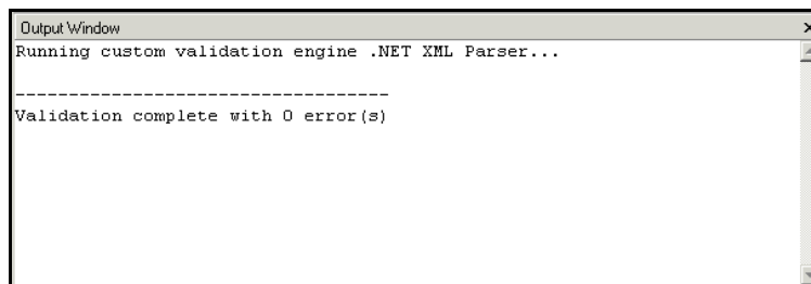
Figure 540. Output Window
