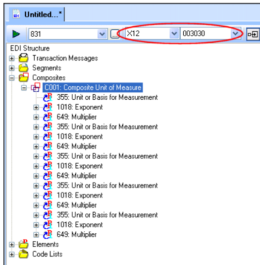
Figure 209. Full Specification
