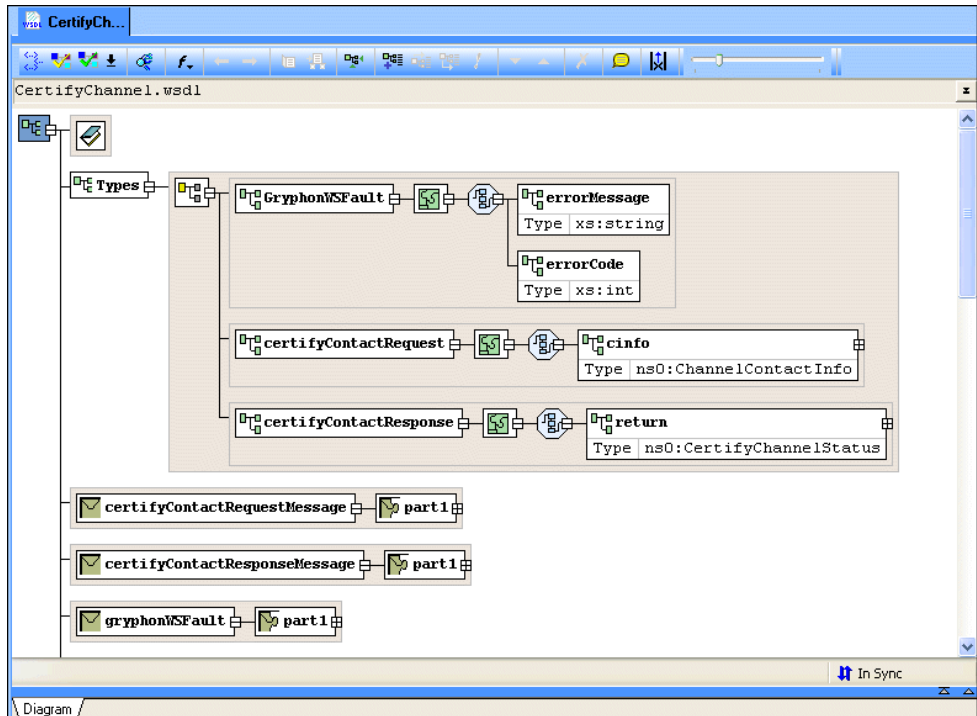
Figure 408. WSDL Diagram Pane
