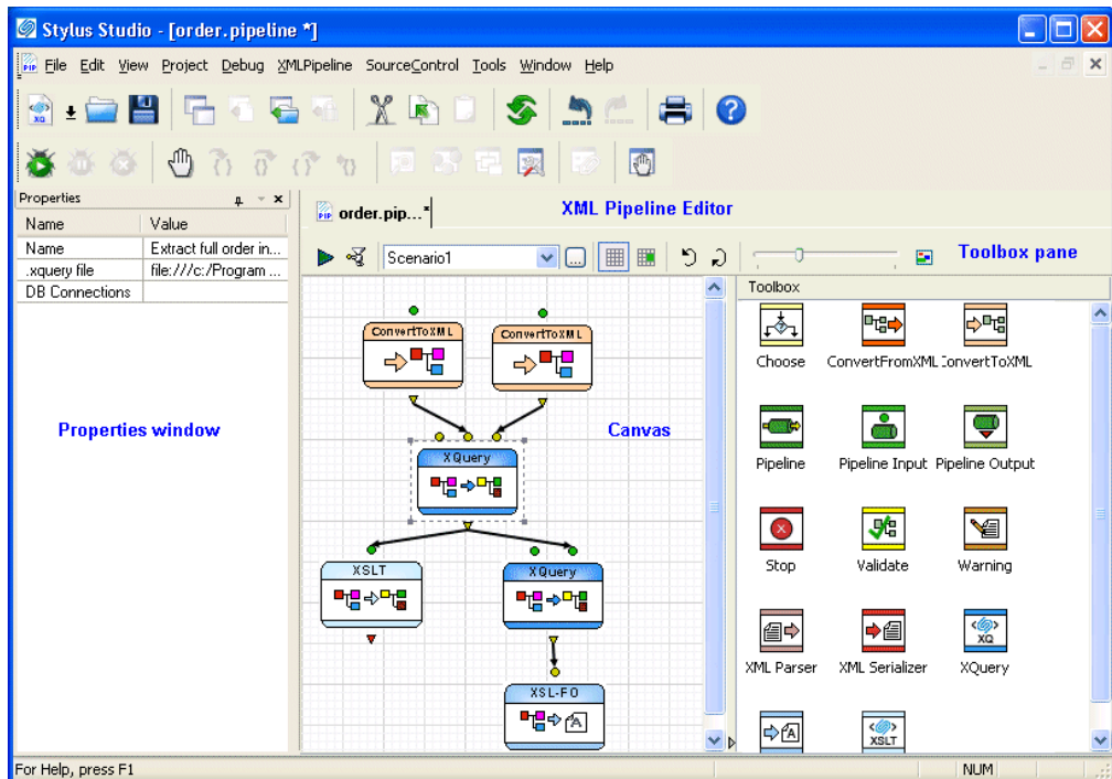
Figure 420. Example of an XML Pipeline in the XML Pipeline Editor
