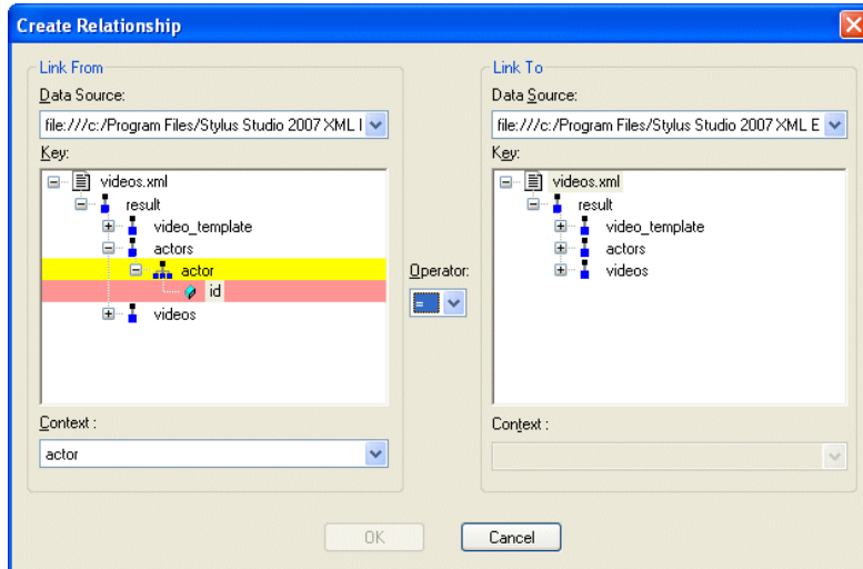
Figure 477. Create Relationship Dialog Box
